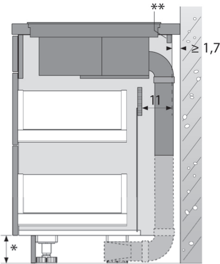
TV... Guided air circulation
